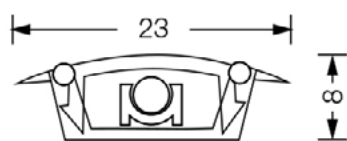
Innfelling
